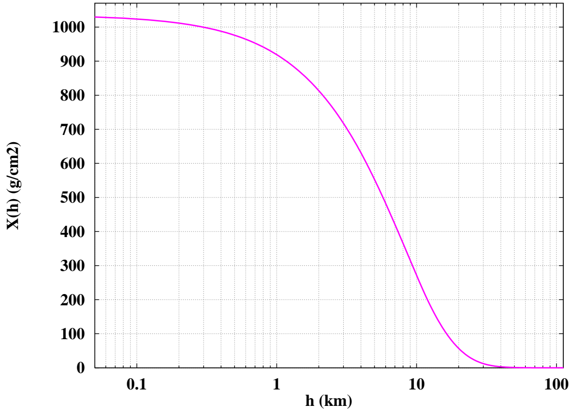
Figure 2.4. Vertical atmospheric depth, X_v , versus vertical altitude over sea level, h , accordingly with Linsley's model [21].
