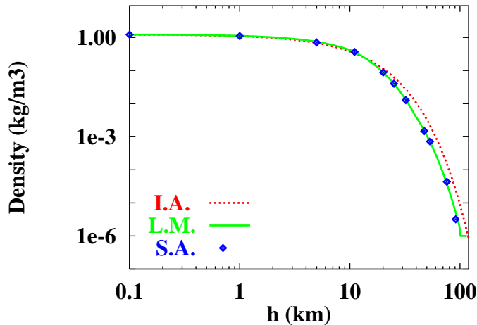
Figure 2.3. Density of the air as a function of the vertical altitude. The dots represent the US standard atmosphere data [19], while the full green line corresponds to Linsley's model [21] and the dashed red one to the isothermal atmosphere \rho(h) = \rho_0 e^{-gMh/RT} with \rho_0 = 1.225 \text{ kg/m}^3 , M = 28.966 and T = 288 \text{ K} .
