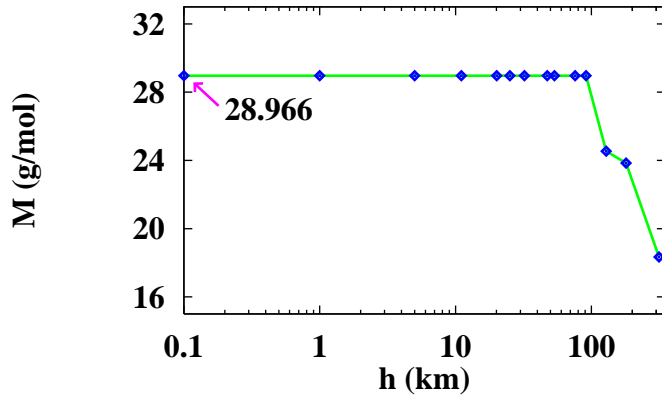
Figure 2.2. Mean molecular weight of the atmosphere as a function of the vertical altitude (US standard atmosphere [19]). The line is only to guide the eye.
